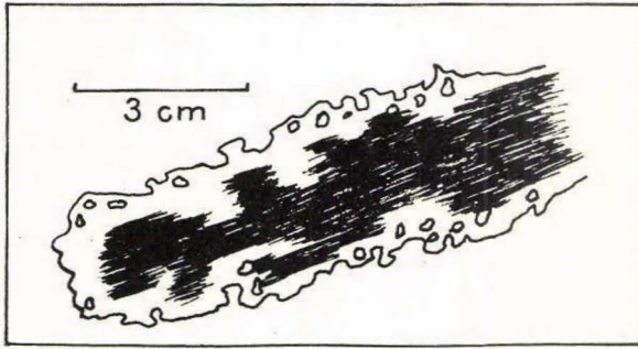
Fig. 13. Sketch of one of the large crystals of soda-amphibole (black) intergrown and replaced by aegirine (unshaded) in a pegmatite in the Malenejfeld Granite. (T.C.R.P.).
