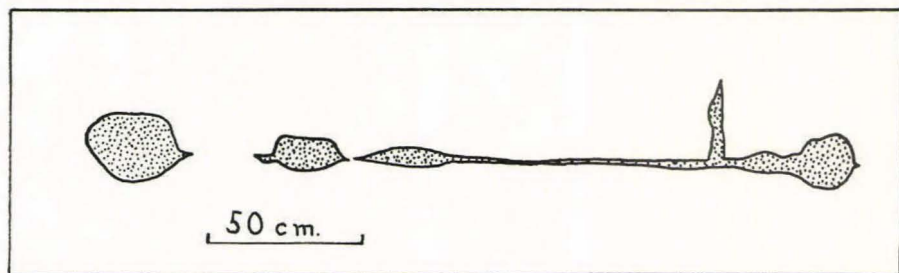
Fig. 5. Mafic "veins" in the Nunarssuit Syenite swelling into bulbous areas. East of the entrance to Eqatdiartarfik. Drawn from a field sketch. (T.C.R.P.).
