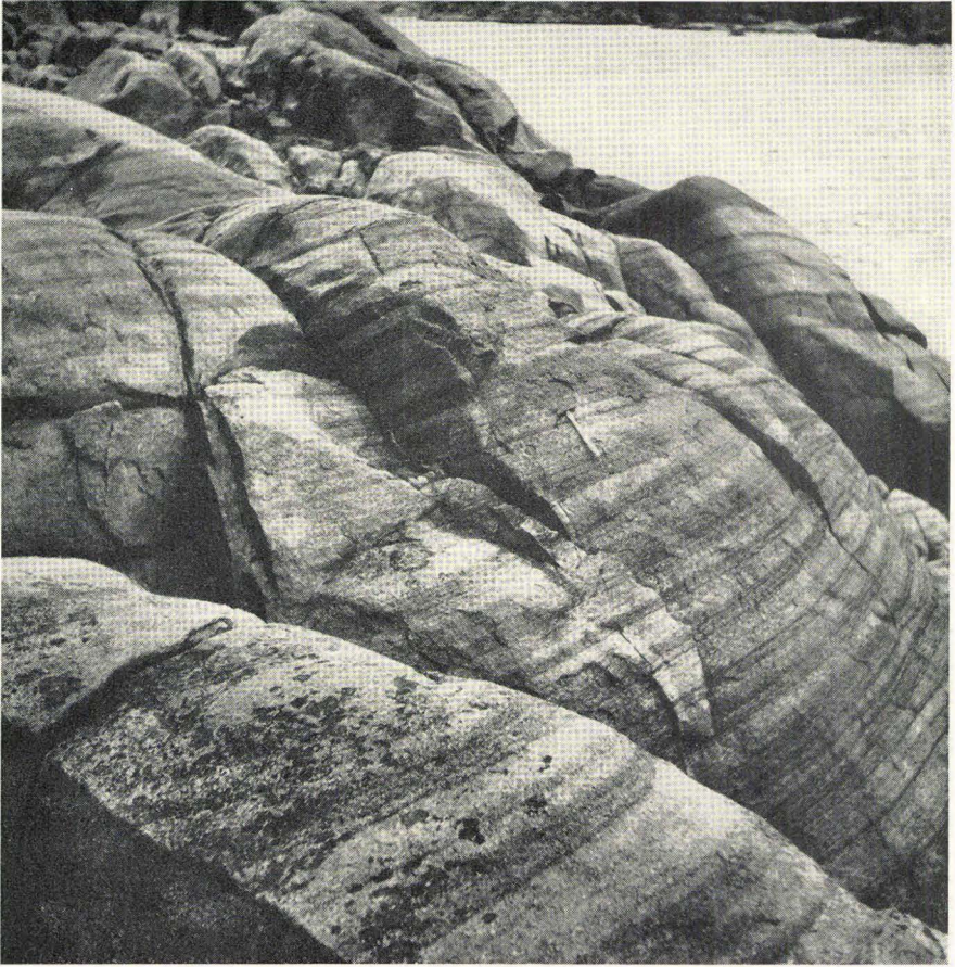
Fig. 51. Well-developed plane-parallel rhythmic mafic layering in the Nunarssuit Syenite on the north side of Tasiussaḡ, Nunarssuit. The hammer handle is 50 cm long. (Photo G.G.U., T.C.R.P.).
