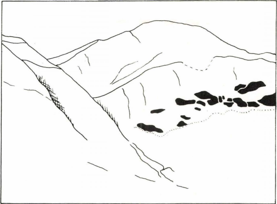
Fig. 22. Key to fig. 21. The metavolcanic lenses are indicated in solid black. The contacts of the Kitdlavât Granite are also drawn in. (T.C.R.P.).
