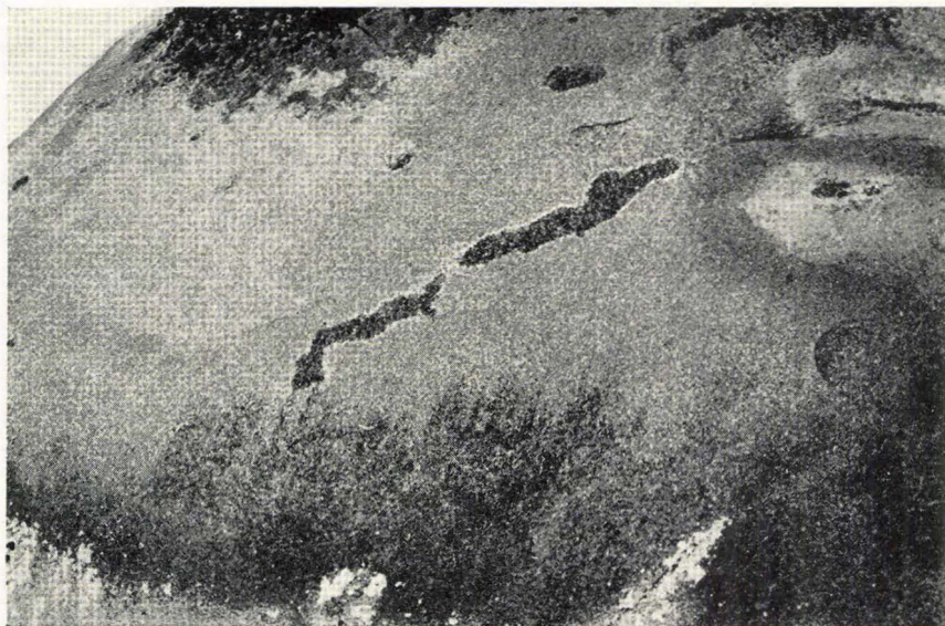
Fig. 4. Mafic clots with leucocratic rims. Nunarssuit Syenite, northern shore of Torssukátak, about 1 km west of Graahs Havn. (Photo G.G.U., W.T.H.).
