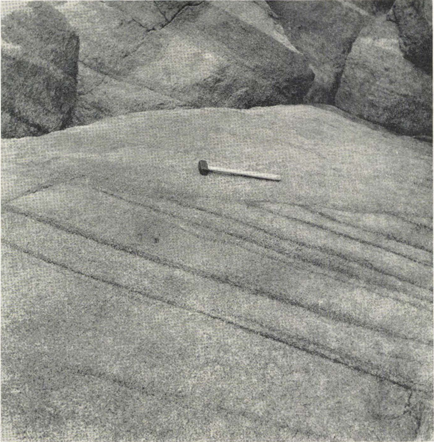
Fig. 55. Angular discordance resulting from the truncation of mafic bands by a thin layer which marks the base of the superincumbent series of layers. Nunarssuit Syenite; on the north side of the entrance to Tasiussaq. (Photo G.G.U., T.C.R.P.).
