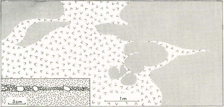
Fig. 18. Medium-grained syenite (stippled) penetrated and enclosed by quartz-poor Helene Granite. Note the round form of the syenite inclusions. The inset shows a thin vein of de-silicated Helene Granite in syenite, with large felspars which cannot have been carried in if the vein were injected in its present form. Drawn from a photograph assisted by field sketches. (T.C.R.P.).
