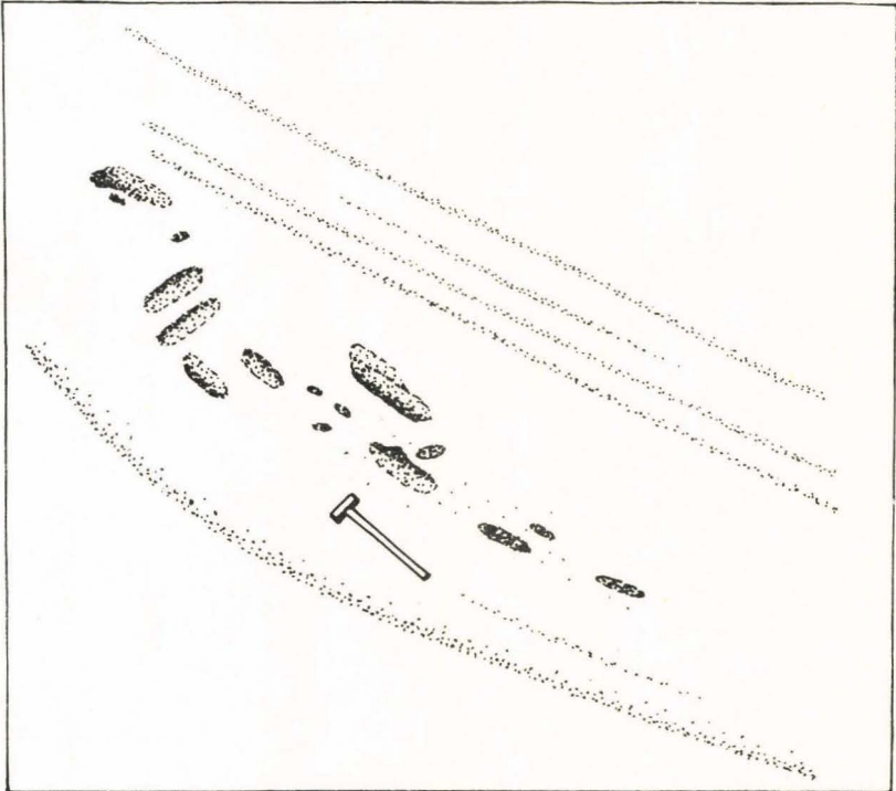
Fig. 61. Slump breccia in the Nunarssuit Syenite south of the entrance to Tasiussaqa. The fragments in the breccia are of banded and gravity stratified syenite which was broken up during strong disturbances. Drawn from a field sketch. (T.C.R.P.).
