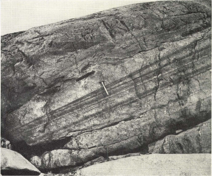
Fig. 60. Concordant breccia zone in banded Nunarssuit Syenite: north of the entrance to Tasiussaqa. The hammer handle is 50 cm long. A block in the breccia about 60 cm above and a little to the left of the head of the hammer can be seen to contain a richly mafic band, showing that the mafic fragments are derived from banded syenite. (Photo G.G.U., T.C.R.P.).
