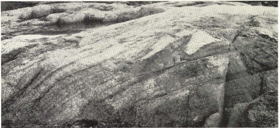
Fig. 31. Moderately inclined planar layering in Helene Granite, near the western shores of Alángorssuaq opposite Quiartorfik. The notebook (right centre) is 17 cm long. (Photo G.G.U., W.T.H.).
