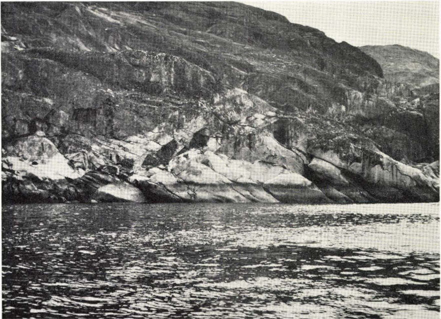
Fig. 10. Eastward-dipping sheet of leucocratic syenite containing metavolcanic inclusions. In the Nunarssuit Syenite on the southern shore of Torssukátak 500 m east of Mercurius Havn. (Photo G.G.U., T.C.R.P.).
