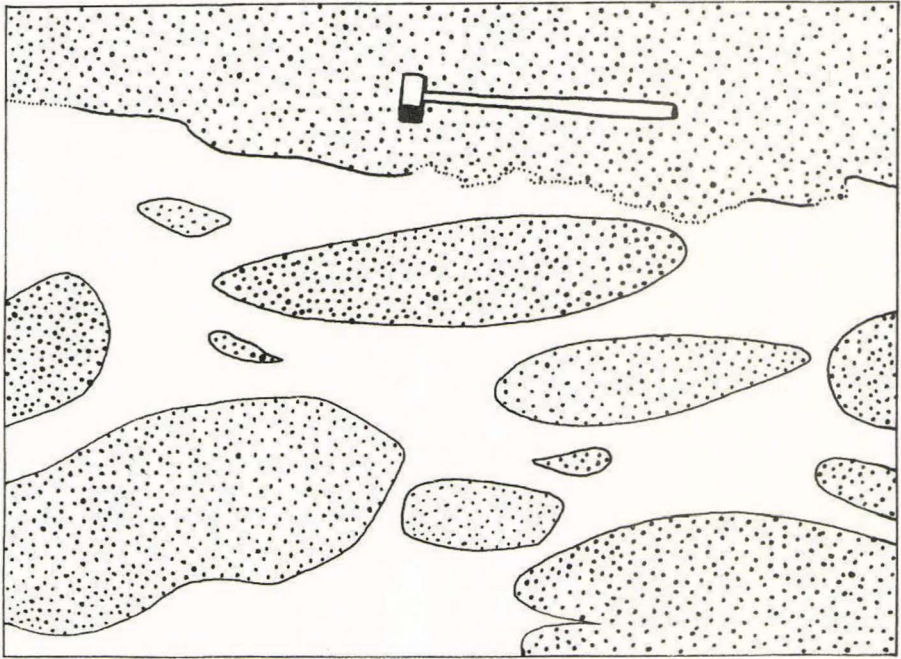
Fig. 9. Rounded-oval inclusions of porphyritic Nunarssuit Syenite in the upper part of the leucocratic sheet north of the entrance to Tasiussaġ. Drawn from a photograph. (T.C.R.P.).
