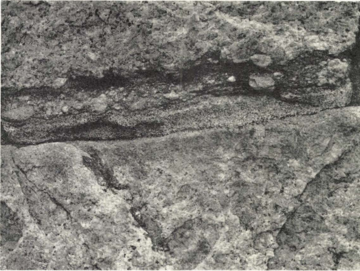
Fig. 46. Close-up of layering in the Helene Granite at the same locality as fig. 44, showing from the bottom upwards, on the left-hand side of the photograph: normal granite passing upwards into microgranite, a thin sharply defined mafic layer, microgranite, a thin mafic layer overlain by a vague zone with large feldspars followed by a thicker mafic layer and normal granite. Note how the thin mafic layer a few mm thick in the middle of the left-hand part of the photograph is depressed beneath superincumbent feldspar phenocrysts several cm long. Similar though less pronounced effects are seen under the small feldspars at the base of the uppermost normal granite layer near the left-hand margin of the photograph. (Photo G.G.U., W.T.H.).
