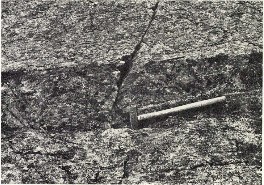
Fig. 6. Pyriclasite sill in quartzo-felspathic hypersthene gneiss showing slight discordancy to the foliation of the gneiss. Quartzo-felspathic streaks in the pyriclasite are parallel to the gneiss foliation.
