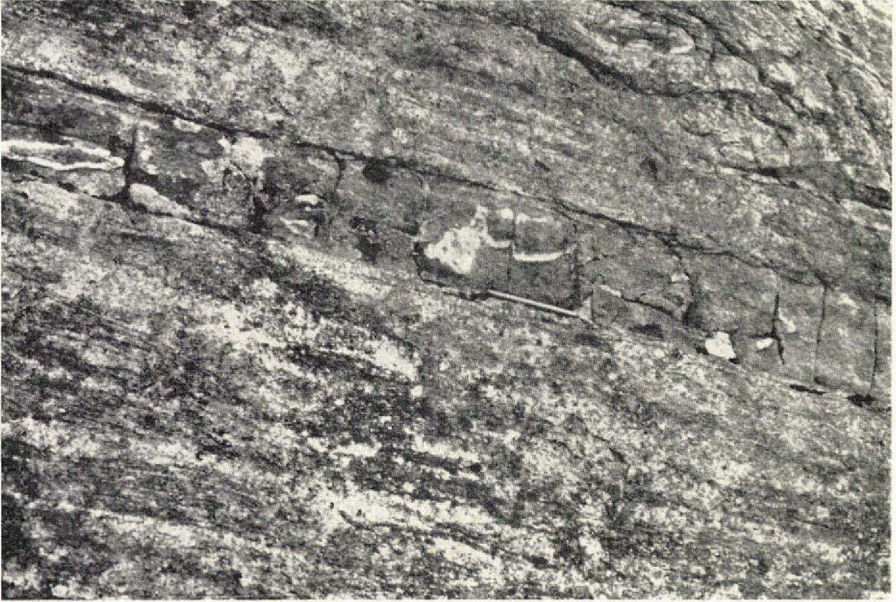
Fig. 3. Pyriclasite sill within hypersthene-garnet gneiss. The sill has sharp contacts to the gneiss and tension cracks have developed in the basic rock, not in the gneiss.
