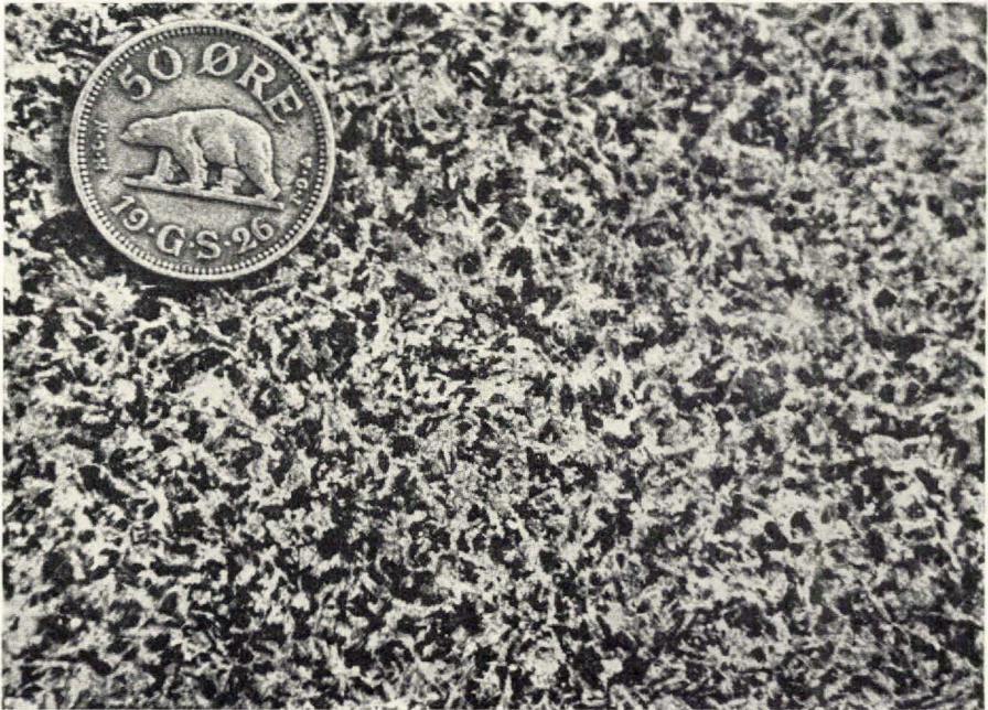
Fig. 13. Texture of metagabbro (3rd episode basic intrusion). The primary pyroxene has been partially replaced by hornblende but with the preservation of the ophitic texture. Diameter of the coin 2.2 cm. Photo: PREBEN CHRISTENSEN.
