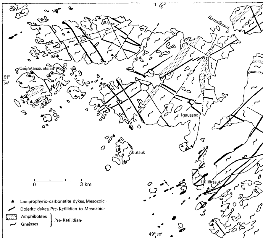
Fig. 1. Outline geology of the Ilulárssuk area.
