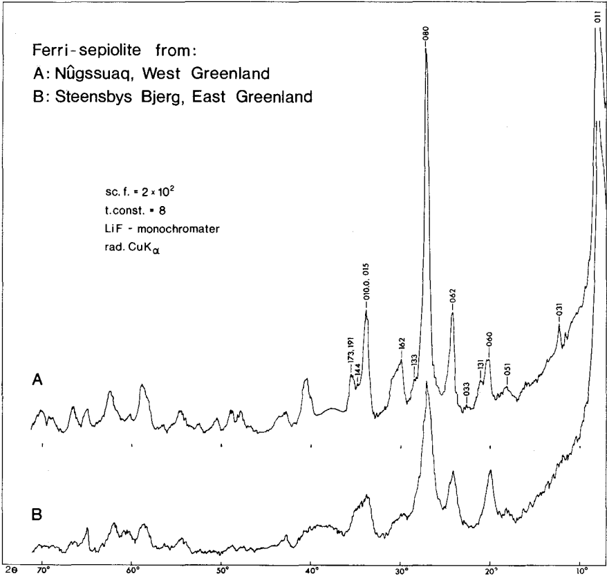
Fig. 3. X-ray diffractometer diagrams of ferri-sepiolite.
