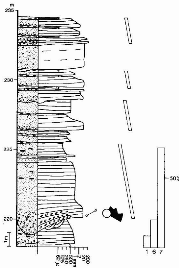
Section 28. Inner fan channel association. South side of Niesen, north Wollaston Forland. Rigi Member; Ryazanian (?).
