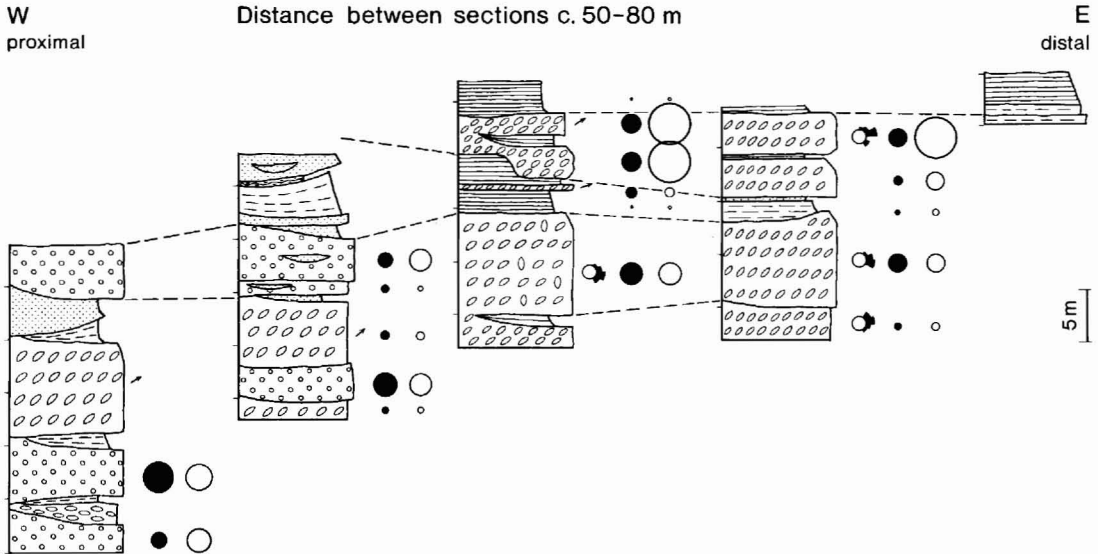
Fig. 39. Correlation between 29–33 (Appendix). Note the extreme lenticularity of all beds. No single beds can be followed between two sections, but major conglomeratic or sandy portions can be correlated (stippled line). The sections are measured in a direction at a right angle to depositional strike. There is no systematic downslope changes in clast size or palaeocurrent direction over the approximately 300 m covered by the section line. Rigi Member, Volgian-Ryazanian.
