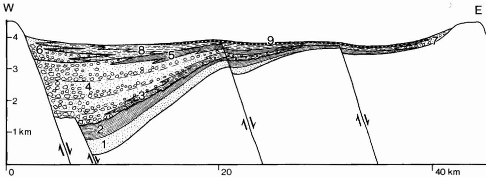
Fig. 4. W-E cross-section through northern Wollaston Forland restored to early Cretaceous situation. 1: Vardekløft Formation (Middle Jurassic), 2: Bernbjerg Formation (Upper Oxfordian-Lower Kimmeridgian). 3-5: Lindemans Bugt Formation (Middle-Upper Volgian); 3: Laugeites Ravine Member, 4: Rigi Member, 5: Niesen Member. 6-9: Palnatokes Bjerg Formation (Ryazanian-Valanginian); 6: Young Sund Member, 7: Falskebugt Member, 8: Albrechts Bugt Member, 9: Rødryggen Member.
