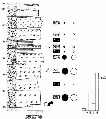
Section 22. Inner fan channel association. Niesen, north Wollaston Forland. Rigi Member; Volgian.
