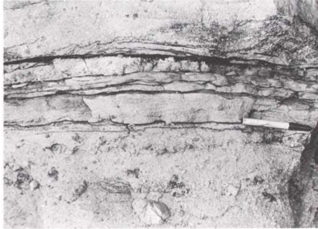
Fig. 29. Stratified pebble conglomerate overlain by horizontally laminated and small scale cross laminated sandstone with mud flasers. Rigi Member, section 44 (Appendix), Clavering Ø, altitude 380 m.
