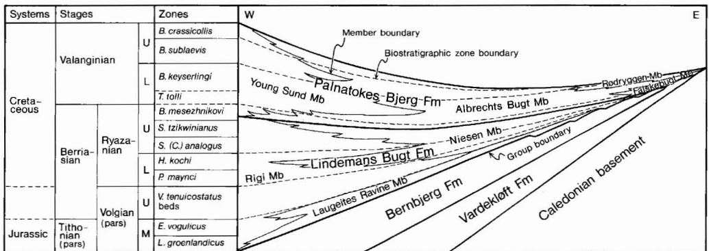
Fig. 1. Stratigraphic scheme of the Middle Volgian – Valanginian sedimentary rocks of the Wollaston Forland Group, East Greenland.
