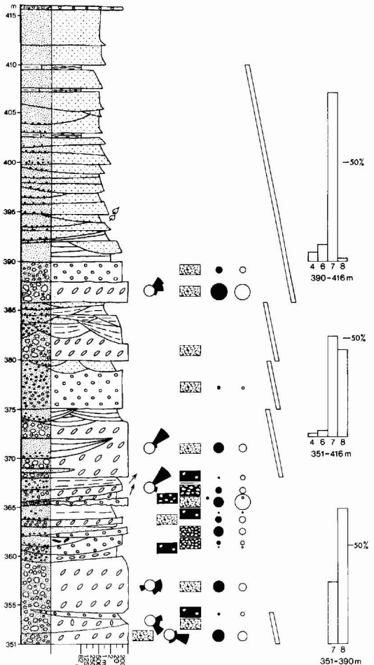
Section 50. Inner fan channel association up to 390 m, where there is a sharp change to the midfan association. NW side of Palnatokes Bjerg, north Wollaston Forland. Rigi Member; Upper Ryazanian. Note the systematic change in palaeocurrent as in section 49.
