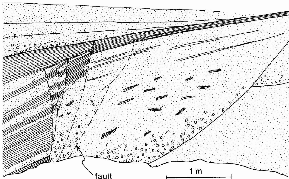
Fig. 40. Synsedimentary slumping along curved scars of channel margin. Deeper part of channel to the left of the figure. Channel mainly filled with mudstone. Section 34 (Appendix) half way up the right section. Rigi Member, south side of Niesen, north Wollaston Forland. Inner fan interchannel association.
