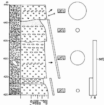
Section 28. Inner fan channel association. South side of Niesen, north Wollaston Forland. Rigi Member; Ryazanian (?).
