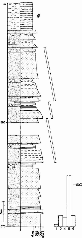
Section 18 5 . Midfan association dominated by fining-upwards cycles. Young Sund Member; Valanginian.
