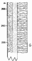
Section 18 3 . Midfan – outer fan transition. Albrechts Bugt Member interfingering with Young Sund Member; Valanginian.
