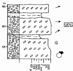
Section 21. Inner fan channel association. Niesen, north Wollaston Forland. Rigi Member; Middle Volgian.
