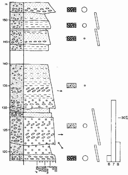
Section 23. Proximal part of midfan association. Niesen, north Wollaston Forland. Rigi Member; Volgian (?).
