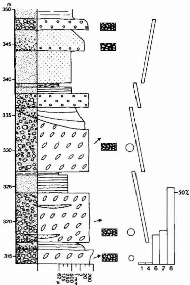
Section 15 4 . Inner fan channel association. Rigi Member; Upper Ryazanian. Sequence somewhat more channelled than shown (see remarks to section 15 3 ).
