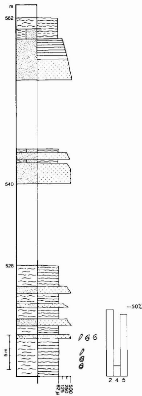
Section 18 4 . Midfan – outer fan transition. Interfingering Albrechts Bugt and Young Sund Members; Valanginian.
