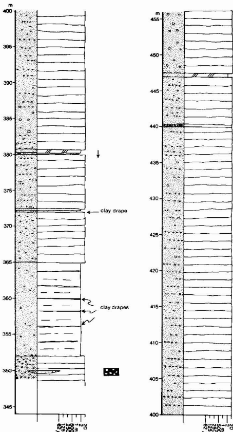
Section 44 1 . Clavering Ø association (facies association c). Coastal section, east Clavering Ø, Rigi Member (?). Volgian–Ryazanian(?).
