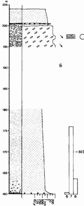
Section 14 2 . Transition between inner fan channel and midfan association. Rigi Member; Lower Ryazanian.
