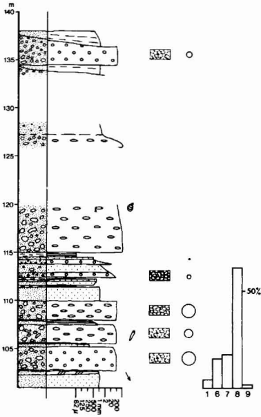
Section 14 1 . Inner fan channel association. Niesen, north Wollaston Forland. Rigi Member; Volgian.
