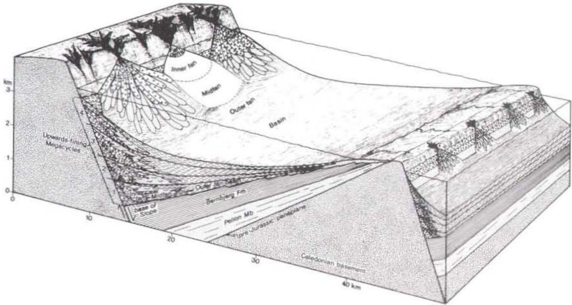
Fig. 41. Block diagram constructed to demonstrate the interpreted palaeoenvironments and resulting facies distribution of the Wollaston Forland Group. The clastic wedge is built of four upwards-fining megacycles each of which corresponds to the model shown on fig. 44. The diagram is based on western Wollaston Forland and the fault scarp to the left corresponds to the Dombjerg Fault.
