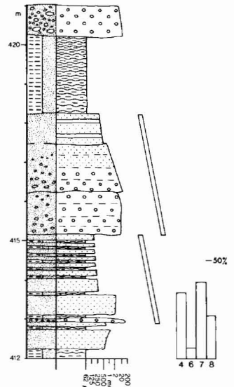
Section 17a. Proximal midfan association. Note the two prominent fining-upwards cycles. Niesen, north Wollaston Forland. Note larger scale than other sections. Rigi Member.
