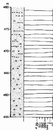
Section 44 3 . As for 44 1 .
