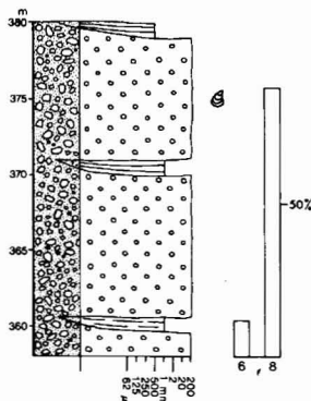
Section 15 5 . Inner fan channel association. Rigi Member; Upper Ryazanian.
