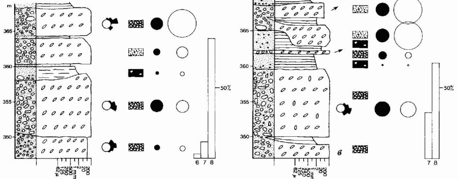
Section 30. Inner fan channel association. See text to section 29. Rigi Member; Volgian-Ryazanian.
