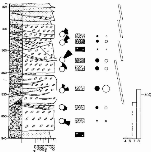
Section 49. Transition from inner fan channel association below to midfan association at 371 m. NW side of Palnatokes Bjerg, north Wollaston Forland. Rigi Member; Upper Ryazanian. Note the systematic trend from E to NE orientated palaeocurrents. The same trend also occurs in the neighbouring section 50.
