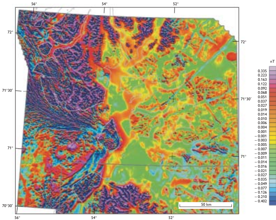
Fig. 3. Calculated vertical gradient of the total magnetic field intensity with shaded relief for the area in central West Greenland covered by project Aeromag 2001 . The location of the aeromagnetic survey in 2001 is circumscribed by a grey line and the new data have been merged with data from project Aeromag 1997 .
