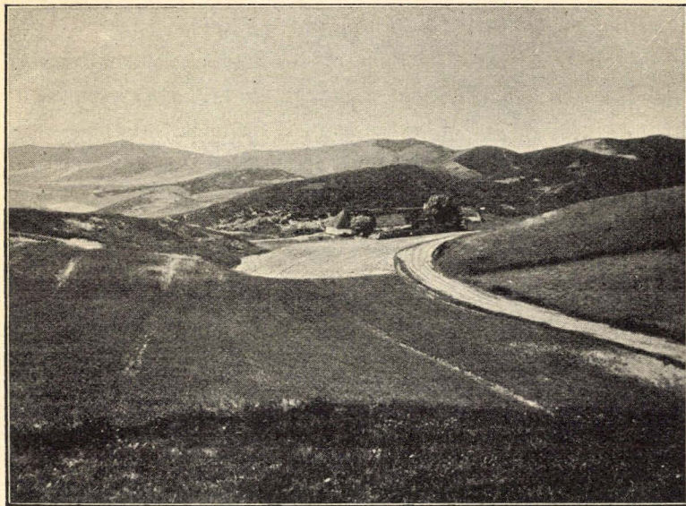
Fig. 1. Bakkerne Syd for Tolne Station.
